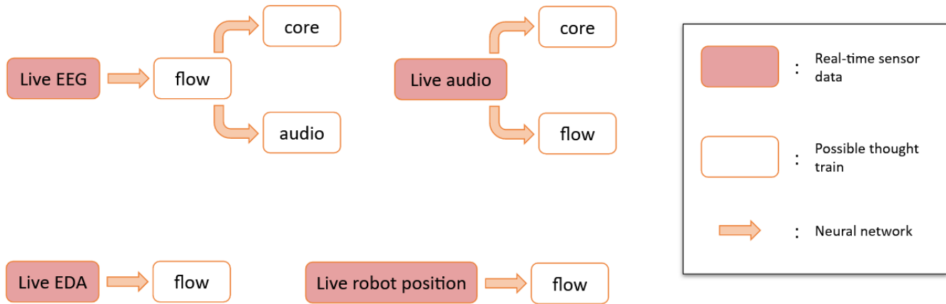
Figure 2: Organisation of the Jess+ AI Factory
