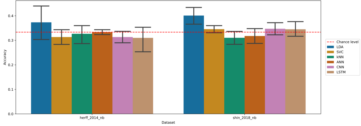
Figure 5.1: Accuracies of the models on the n-back datasets with the subject-independent approach (95% confidence intervals related to the variability on the 5-fold outer cross-validation are displayed).
