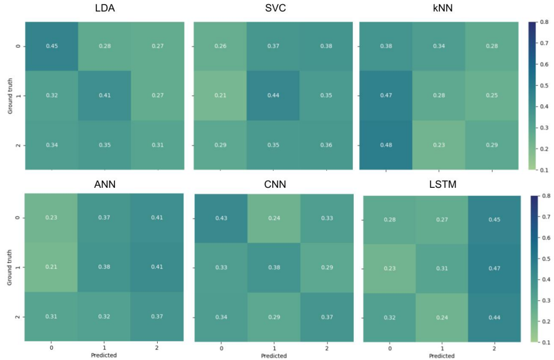
Figure 2: Confusion matrices for the subject-independent approach on the Shin et al. 2018 dataset of n-back tasks. Classes 0, 1 and 2 are 0-, 2- and 3-back respectively.
