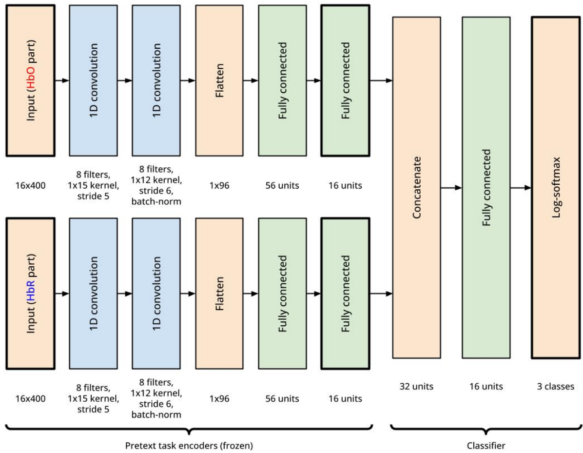
Figure 6.4: Full transfer model architecture.
