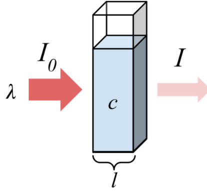
Figure 2.1: Path of the light in a cuvette for which the Beer-Lambert law can be applied simply (Source: commons.wikimedia.org).
