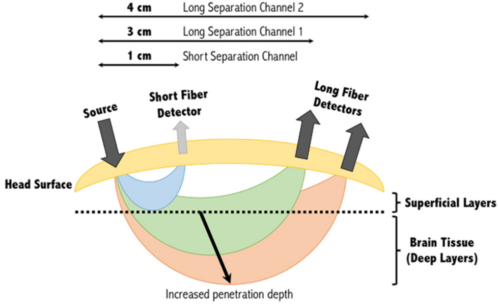
Figure 2.5: Short separation channels ( Source: Rupawala et al., 2018 ).
