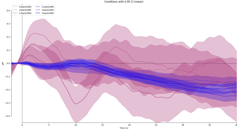
Figure 5.6: Grand average of the epochs of each n-back condition for HbO and HbR. The bands represent the 95% confidence interval related to the variability on the epochs of each condition.
