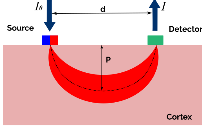
Figure 2.2: Path of the light in the brain with fNIRS for which we can apply the modified Beer-Lambert law ( Source: newmanbrain.com ).
