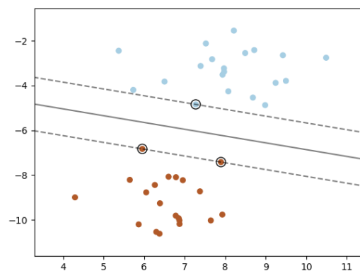
Figure 2.10: Example of linear SVM with two classes, showing the decision boundary and support vectors ( Source: scikit-learn.org ).
