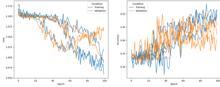
Figure 5.5: Training and validation graphs of the dataset-tailored CNN (cross-entropy loss on the left and accuracy on the right).
