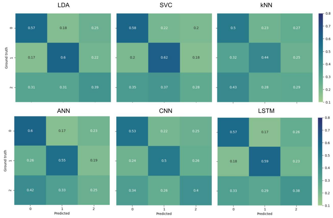
Figure 5: Confusion matrices for the subject-independent approach on the Bak et al. 2019 dataset of motor execution tasks. Classes 0, 1 and 2 are right hand finger tapping, left hand finger tapping and foot tapping respectively.
