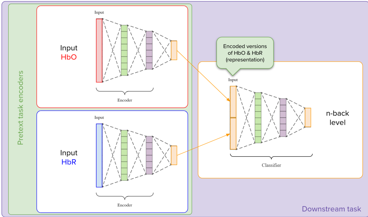
Figure 6.3: Diagram of the concept of transfer learning from the pretext task to the downstream task.
