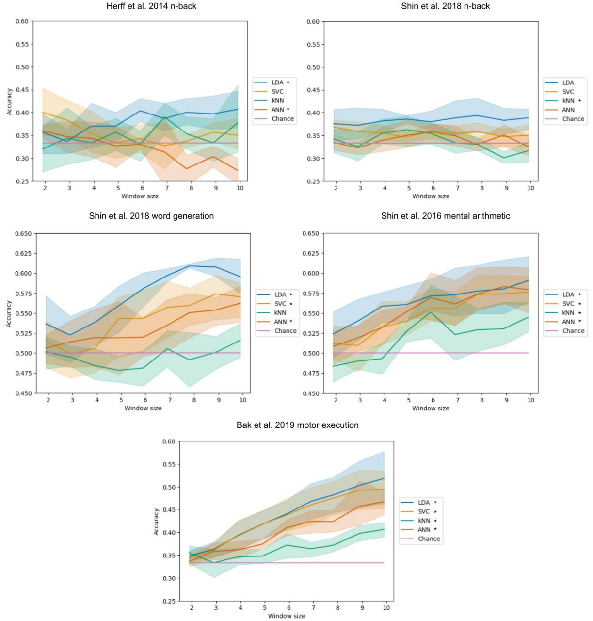
Figure 4.2: Accuracy with respect to the time window length. The bands represent the 95% confidence interval related to the variability on the 5-fold outer cross-validation. Legend entries marked with an asterisk indicate a significant correlation at a 5% threshold.
