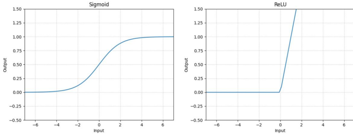
Figure 2.12: Activation functions (sigmoid on the left, rectified linear unit on the right)
