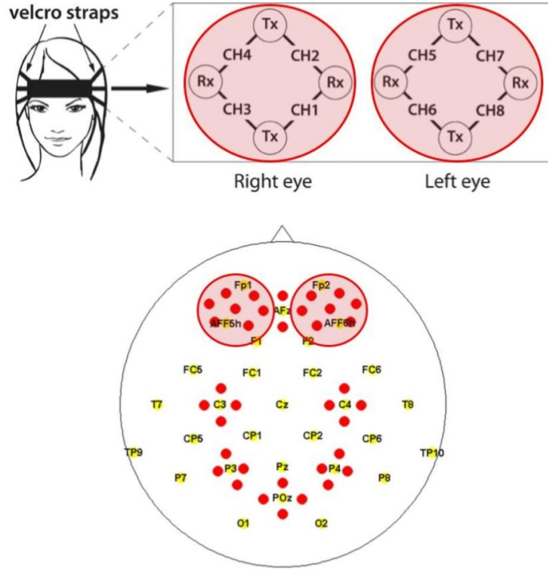
Figure 3.1: Maps of the regions of interest as circled in the red areas. Top : n-back dataset from Herff et al. 2014, fNIRS channels are represented by black lines with CH labels, each region of interest was an averaging of 4 channels. Bottom : n-back and word generation datasets from Shin et al. 2018, fNIRS channels are represented by red dots, each region of interest was an averaging of 7 channels.
