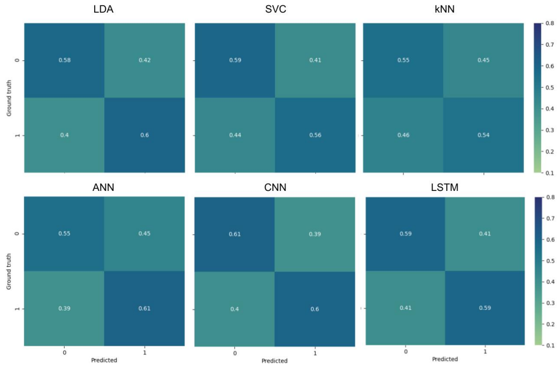
Figure 4: Confusion matrices for the subject-independent approach on the Shin et al. 2016 dataset of mental arithmetic tasks. Classes 0 and 1 are baseline task and mental arithmetic respectively.
