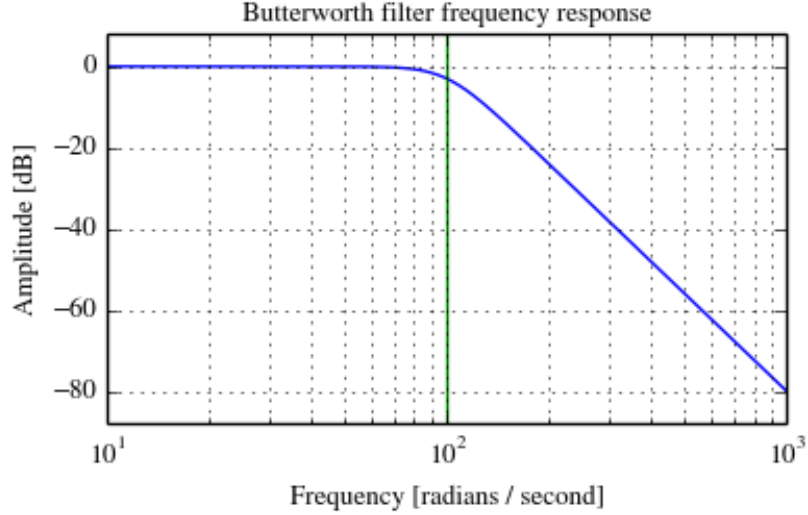
Figure 2.4: Bode plot of a lowpass filter of order 4 with an angular cutoff frequency of 100 \text{ rad.s}^{-1} (Source: docs.scipy.org ).
