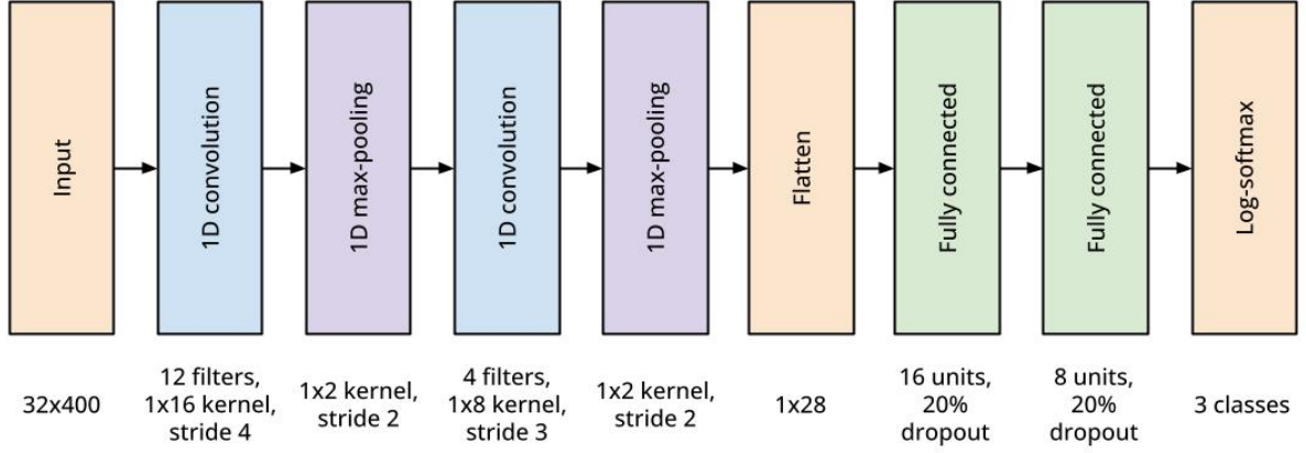
Figure 5.4: CNN architecture.
