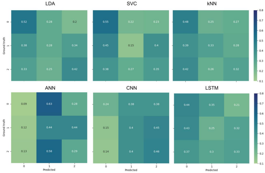
Figure 1: Confusion matrices for the subject-independent approach on the Herff et al. 2014 dataset of n-back tasks. Classes 0, 1 and 2 are 1-, 2- and 3-back respectively.
