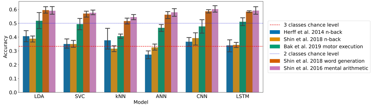
Figure 4.1: Accuracies of the models on each dataset with the subject-independent approach, models are all using HbO and HbR simultaneously (95% confidence intervals related to the variability on the 5-fold outer cross-validation are displayed).
