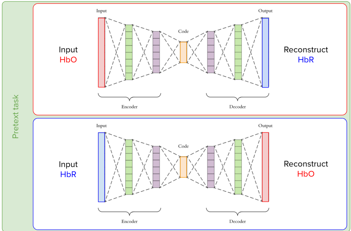
Figure 6.1: Diagram of the concept of representation learning for the pretext task: reconstruction of HbR from HbO, and reconstruction of HbO from HbR.
