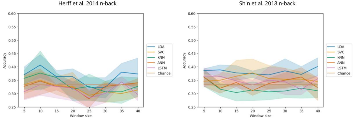
Figure 5.2: Accuracy with respect to the time window length. The bands represent the 95% confidence interval related to the variability on the 5-fold outer cross-validation. Legend entries marked with an asterisk indicate a significant correlation at a 5% threshold.
