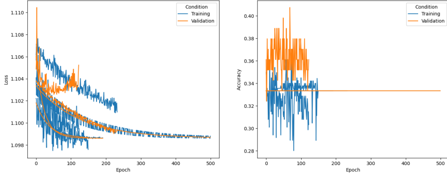
Figure 6.6: Training and validation graphs of the control transfer learning approach with only labelled data (cross-entropy loss on the left and accuracy on the right).
