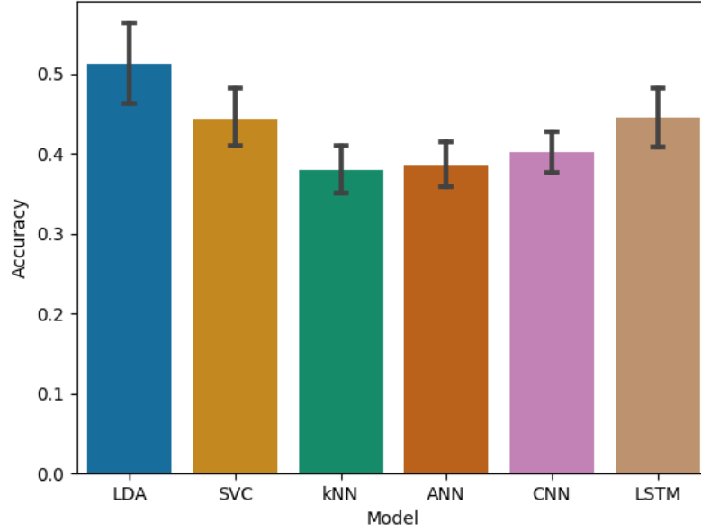
Figure 4.4: Accuracy for the subject-specific approach on the dataset from Bak et al. 2019 of motor execution tasks (95% confidence intervals related to the variability on the subjects are displayed)
