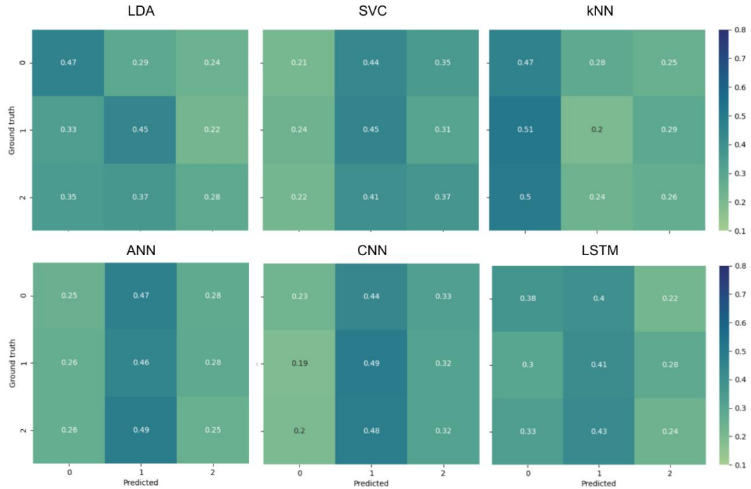
Figure 7: Confusion matrices for the n-back tailored subject-independent approach on the Shin et al. 2018 dataset of n-back tasks. Classes 0, 1 and 2 are 0-, 2- and 3-back respectively.
