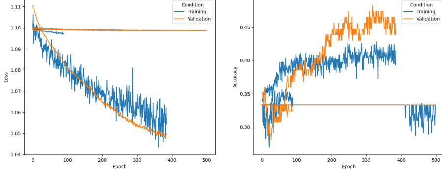
Figure 6.5: Training and validation graphs of the transfer learning approach with both labelled and unlabelled data (cross-entropy loss on the left and accuracy on the right).
