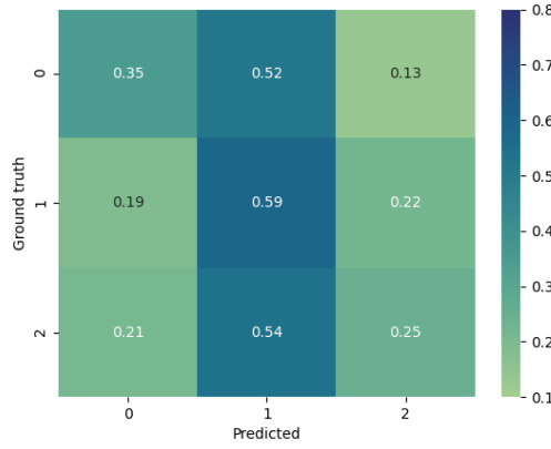
Figure 5.7: Confusion matrix of the CNN tailored to the Shin et al. 2018 dataset of n-back tasks. Classes labelled 0, 1 and 2 represent 0-, 2-, and 3-back respectively.
