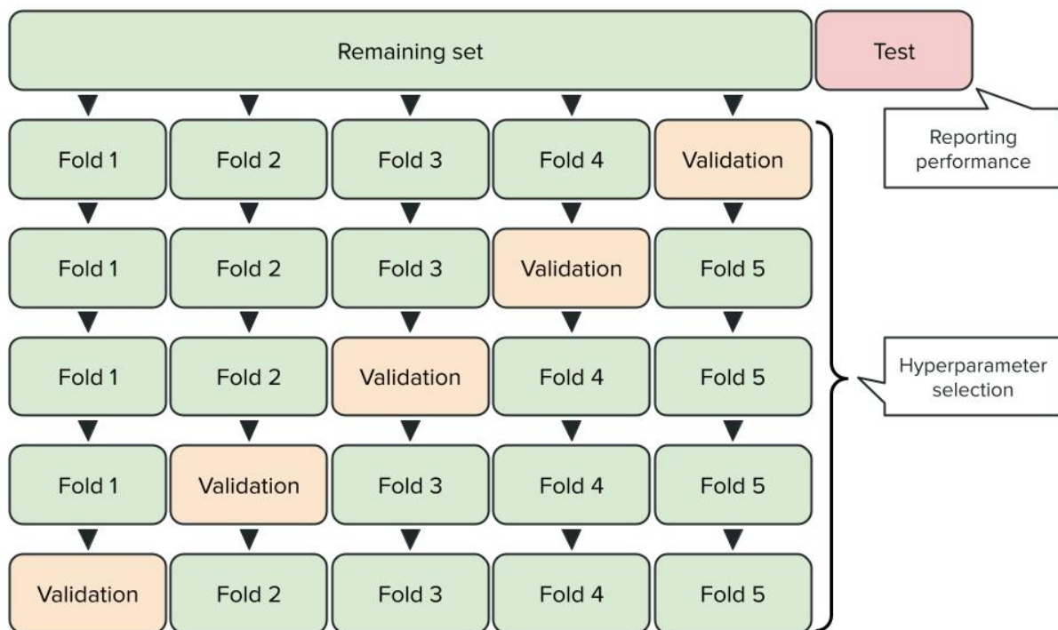
Figure 2.14: Example of inner 5-fold cross-validation.
