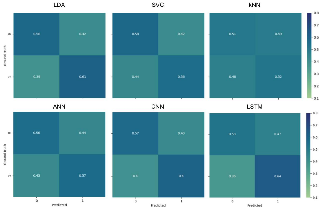
Figure 3: Confusion matrices for the subject-independent approach on the Shin et al. 2018 dataset of word generation tasks. Classes 0 and 1 are baseline task and word generation respectively.
