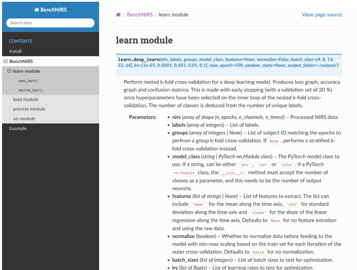
Figure 3.3: Screenshot of the online documentation of a BenchNIRS function.
