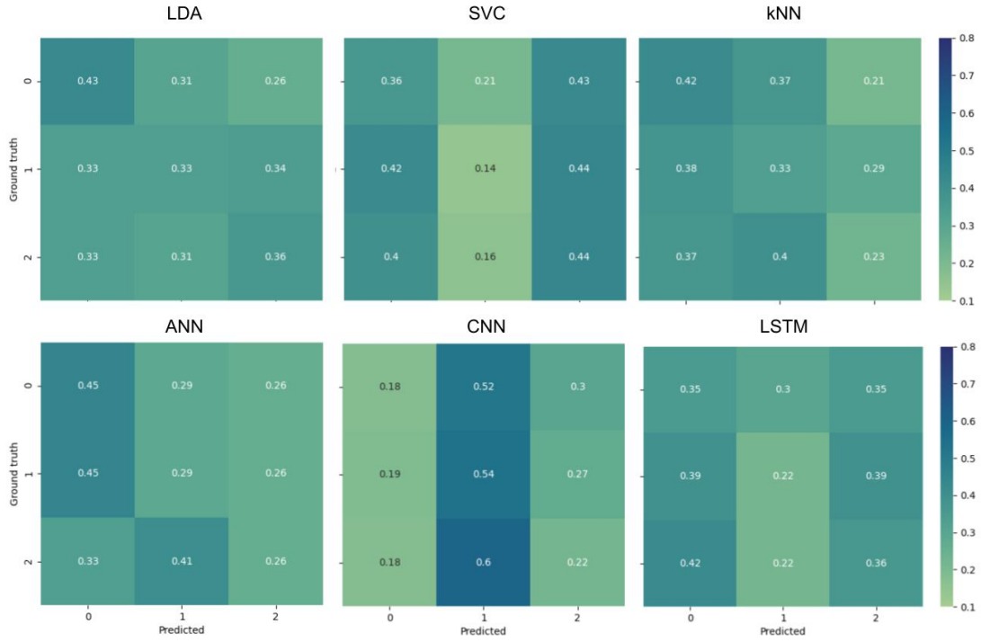
Figure 6: Confusion matrices for the n-back tailored subject-independent approach on the Herff et al. 2014 dataset of n-back tasks. Classes 0, 1 and 2 are 1-, 2- and 3-back respectively.
