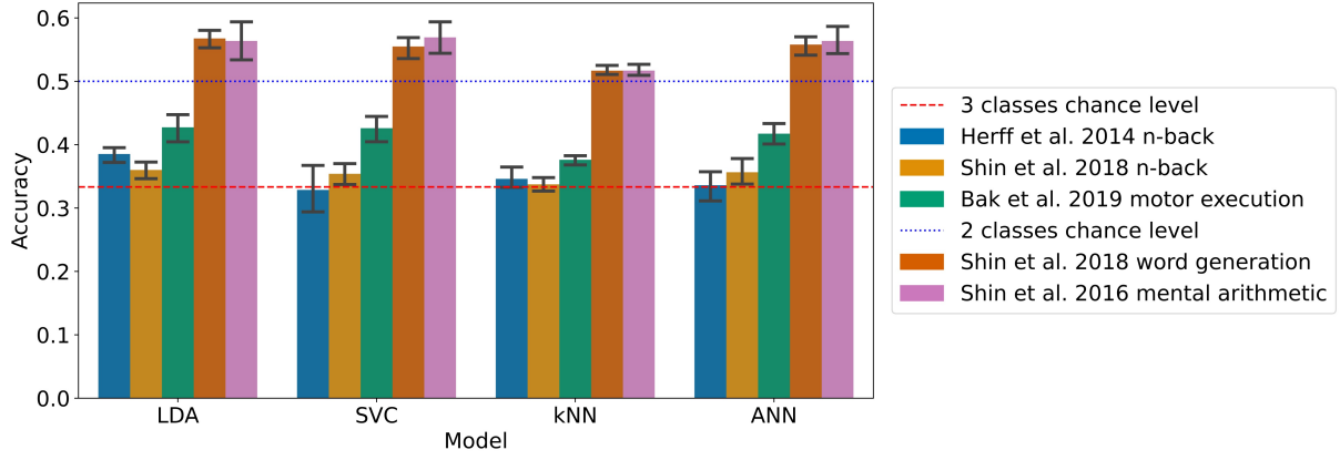
Figure 4.3: Accuracies of the models on each dataset with the subject-independent approach using a 2-second sliding time window, models are all using HbO and HbR simultaneously (95% confidence intervals related to the variability on the 5-fold outer cross-validation are displayed).
